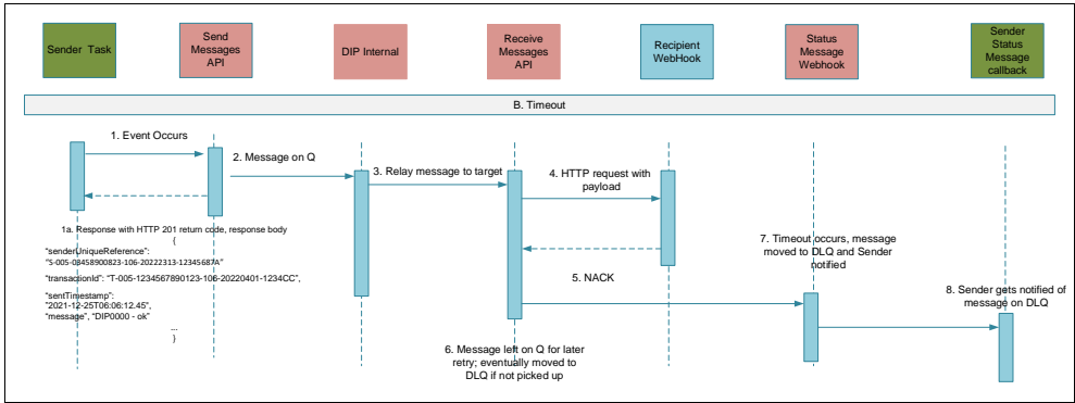
Figure 12 – Recipient Timeout
